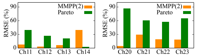
Fig. 4: Comparison of RMSE: OFFICE (left) and HOME (right).
